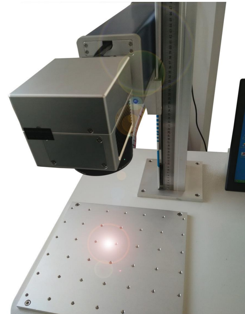
Medium and heavy plate punch marking machine
